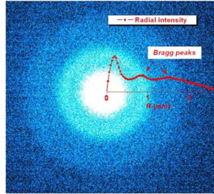
Figure 7. Diffracted beam
