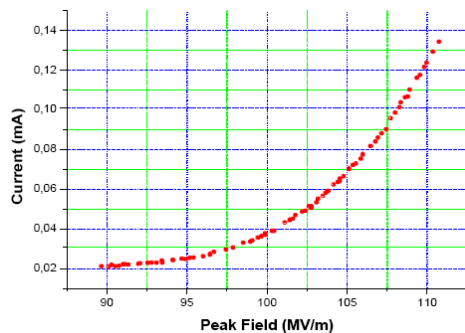
Figure 3. Dark current as a function of peak field in the gun
