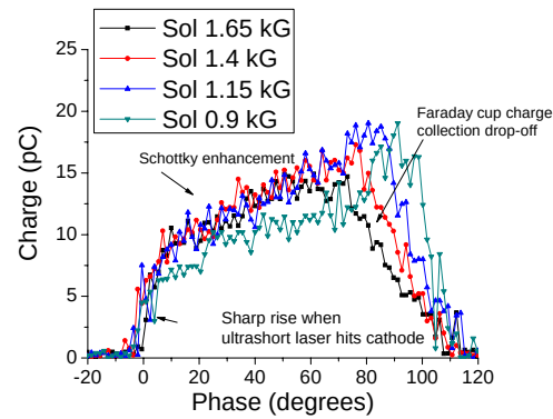
Figure 4. Charge vs phase
