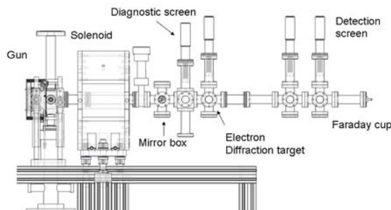
Figure 1. Pegasus beamline layout
