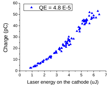
Figure 5. QE measurement
