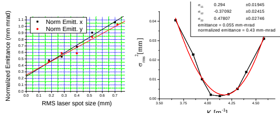
Figure 6. Thermal emittance measurement
