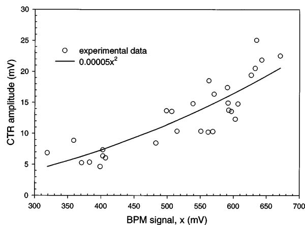
FIG. 4. The transition radiation signal as a function of the total number of electrons. The BPM signal is proportional to the total charge ( eN ) of the electron beam.
